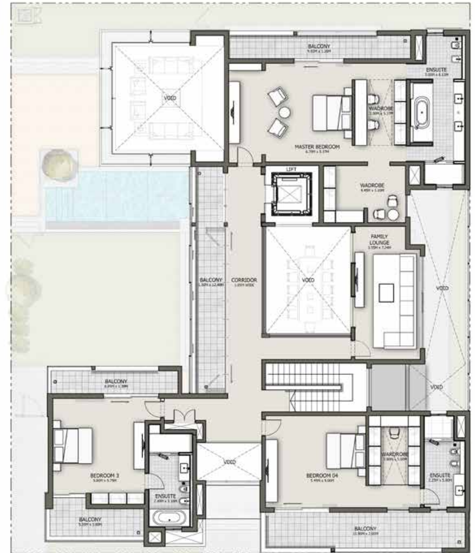
First Floor
